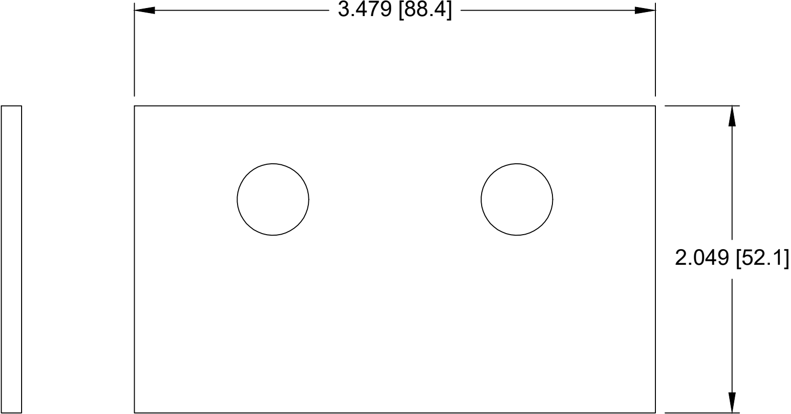
Bracket
