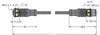
Dimension drawing
