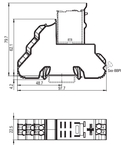
fig. 2. Dimension (mm)
