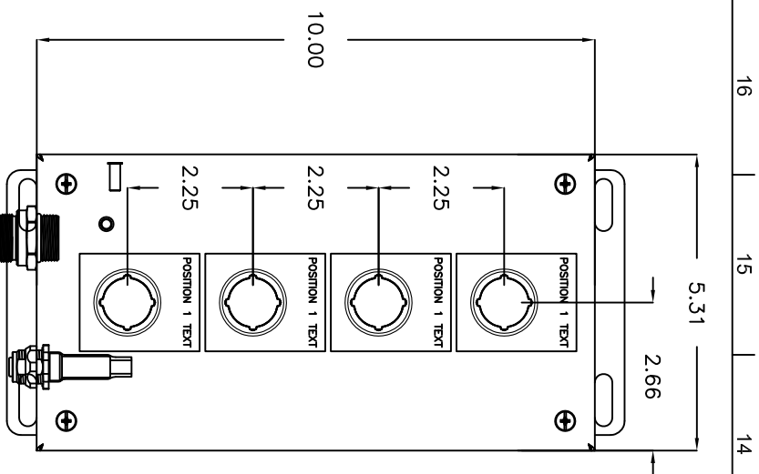
FRONT SIDE VIEW OF ENCLOSURE
