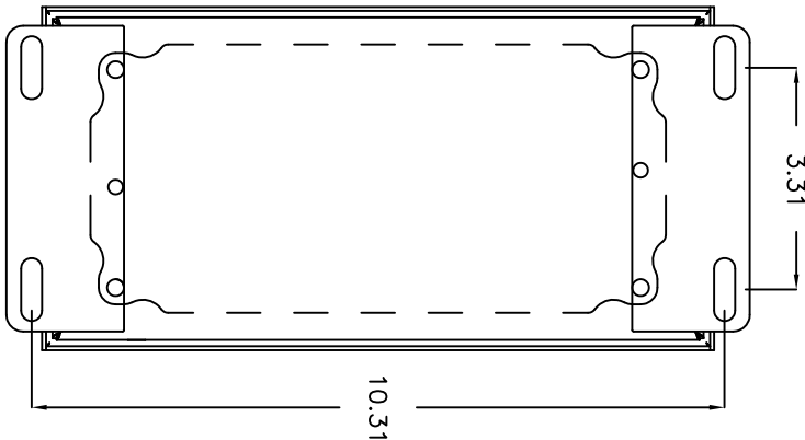
BACK SIDE VIEW OF ENCLOSURE
