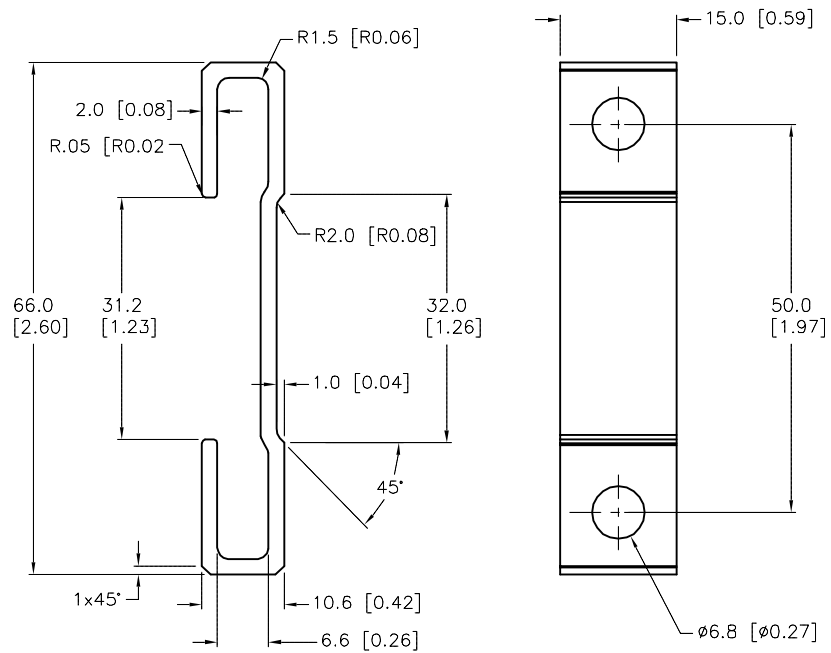
(2x) MOUNTING BRACKET
