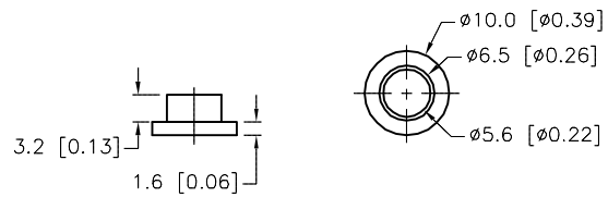
(8x) NYLON SLEEVE
